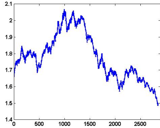
(b) French franc log spot rate
