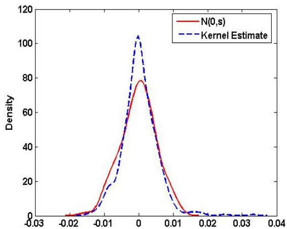
(c) Swedish residuals from VAR(12) ( \alpha = 1.80 )
