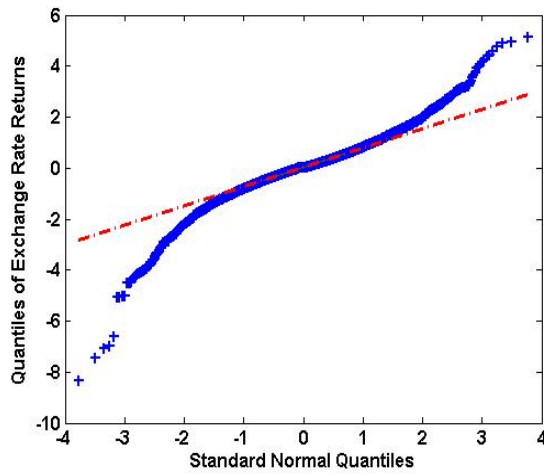
(c) Japanese residuals
