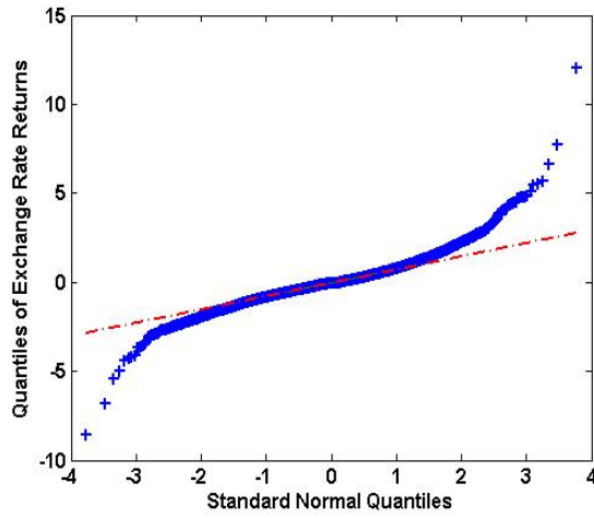
(a) Australian residuals
