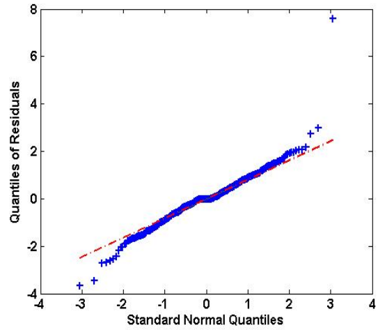
(b) Canadian residuals from VAR(12) ( \alpha = 1.86 )
