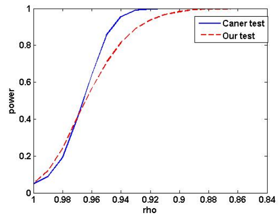
(f) \alpha = 1.9, T = 500
