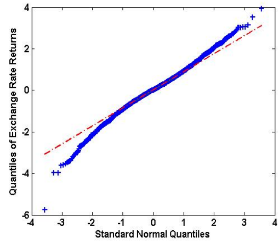
(b) French residuals
